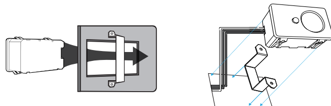
Diagrams show internal cross section of fixture with bracket included for additional sensor impact strength.
